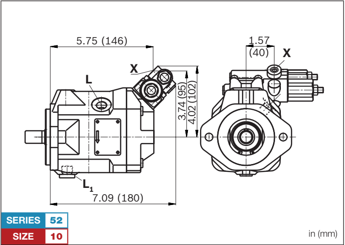
DFR/DFR1 – Pressure, flow controller (metric) 1)
