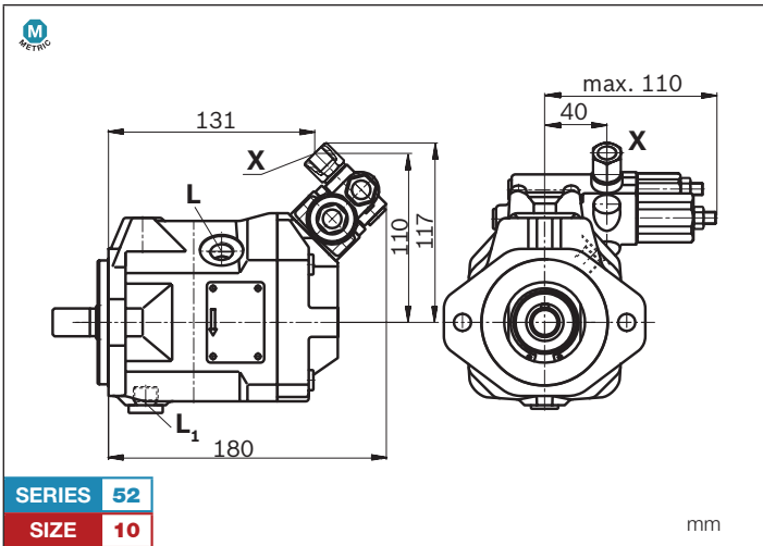
DRG – Pressure controller, remotely controlled (metric) 1)
